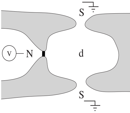
FIG. 1. An Andreev quantum dot formed by a normal conducting cavity ( d ) with two superconducting ( S ) contacts. In the transport state, an infinitesimal voltage V is applied between the grounded superconductors and the normal reservoir ( N ) contacted at the left opening. The distribution of S derived in this paper considers the effect of a tunnel barrier in the normal contact, indicated by a black rectangle in the figure.
