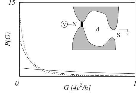
FIG. 2. Conductance distribution for a single mode chaotic Andreev quantum dot in a magnetic field for different values of the barrier transparency \Gamma . A sketch of the system is shown in the inset. The barrier is indicated by a black rectangle. The solid, dashed, and dotted curves correspond to \Gamma=0.9 , \Gamma=0.6 , and \Gamma=0.5 , respectively.
